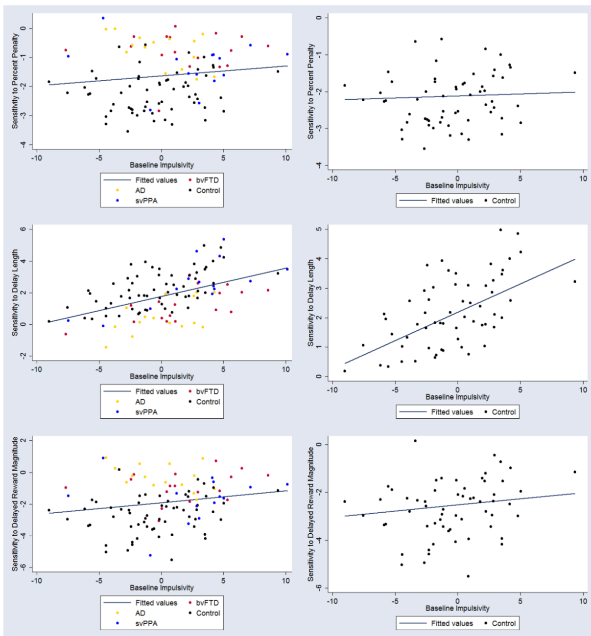
1 Supplementary Figure 3. Scatterplots depicting correlations between estimates produced by the 2 behavioral model. The left column shows these relationships using estimates for all subjects, and the 3 corresponding panel in the right column shows this relationship only in healthy controls.
