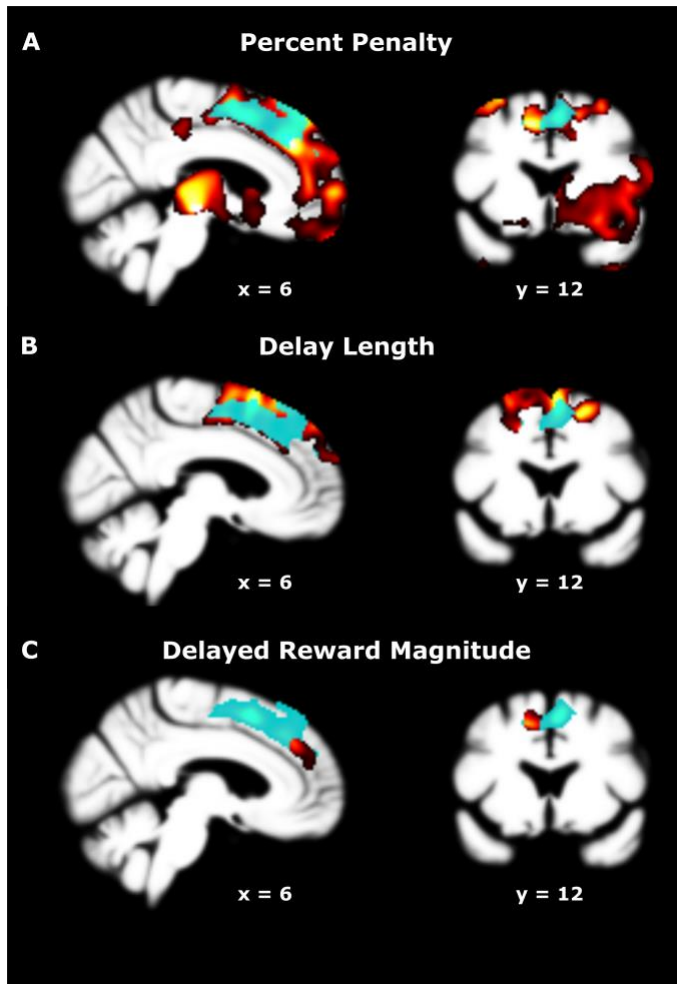
2 Supplementary Figure 5. Conjunction analysis highlighting dmPFC volumes (cyan overlay) that were 3 significantly associated with estimates of sensitivity to all three choice attributes, including (A) percent 4 penalty, (B) delay length, and (C) delayed reward magnitude. Conjunction analysis results are overlaid 5 onto the relevant main brain-behavior correlation findings derived from voxel-based morphometry analyses 6 depicted in Fig. 4 of the main text. Images are oriented by neurological convention.
