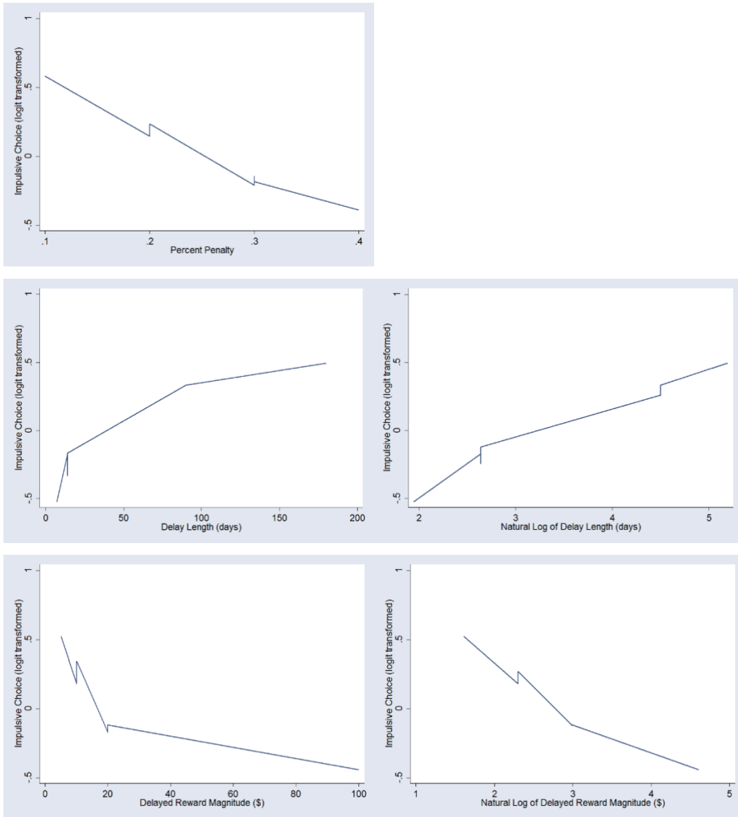
2 Supplementary Figure 2. Locally-weighted logit regressions estimating relationships between values of 3 choice attributes and the log-odds of choosing the smaller immediate reward. The left column shows this 4 relationship for untransformed choice attributes, and the right shows the effect of natural log transformations 5 for delay length and delayed reward magnitude on the linearity of their relationship with the log-odds of 6 choosing the immediate reward.
