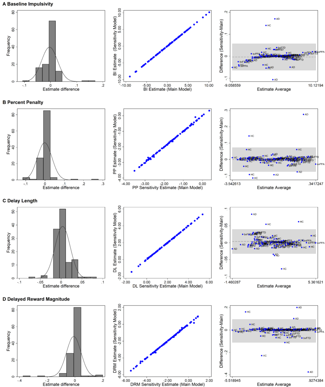
2 Supplementary Figure 6. Sensitivity analysis results excluding one subject with clinical diagnosis of AD 3 but negative amyloid PET imaging. From left to right, a histogram depicting the distribution of differences 4 between the main model and sensitivity analysis model with overlaid normal distribution, scatterplot, and 5 Bland-Altman plot with individual diagnoses for model estimates of (A) baseline impulsivity, and sensitivities 6 to (A) percent penalty, (B) delay length, and (C) delayed reward magnitude.
