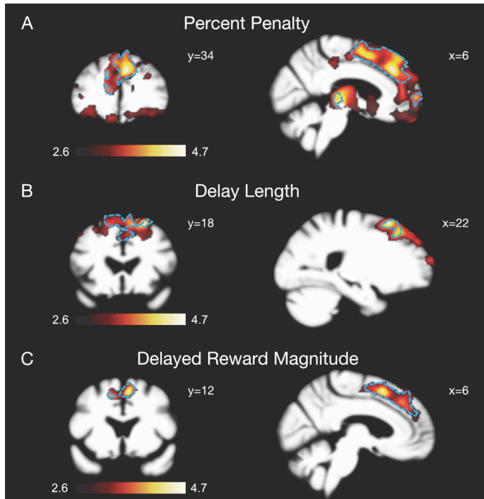
1 Figure 4 Neuroanatomic correlates of sensitivity to information presented in an intertemporal 2 choice.
