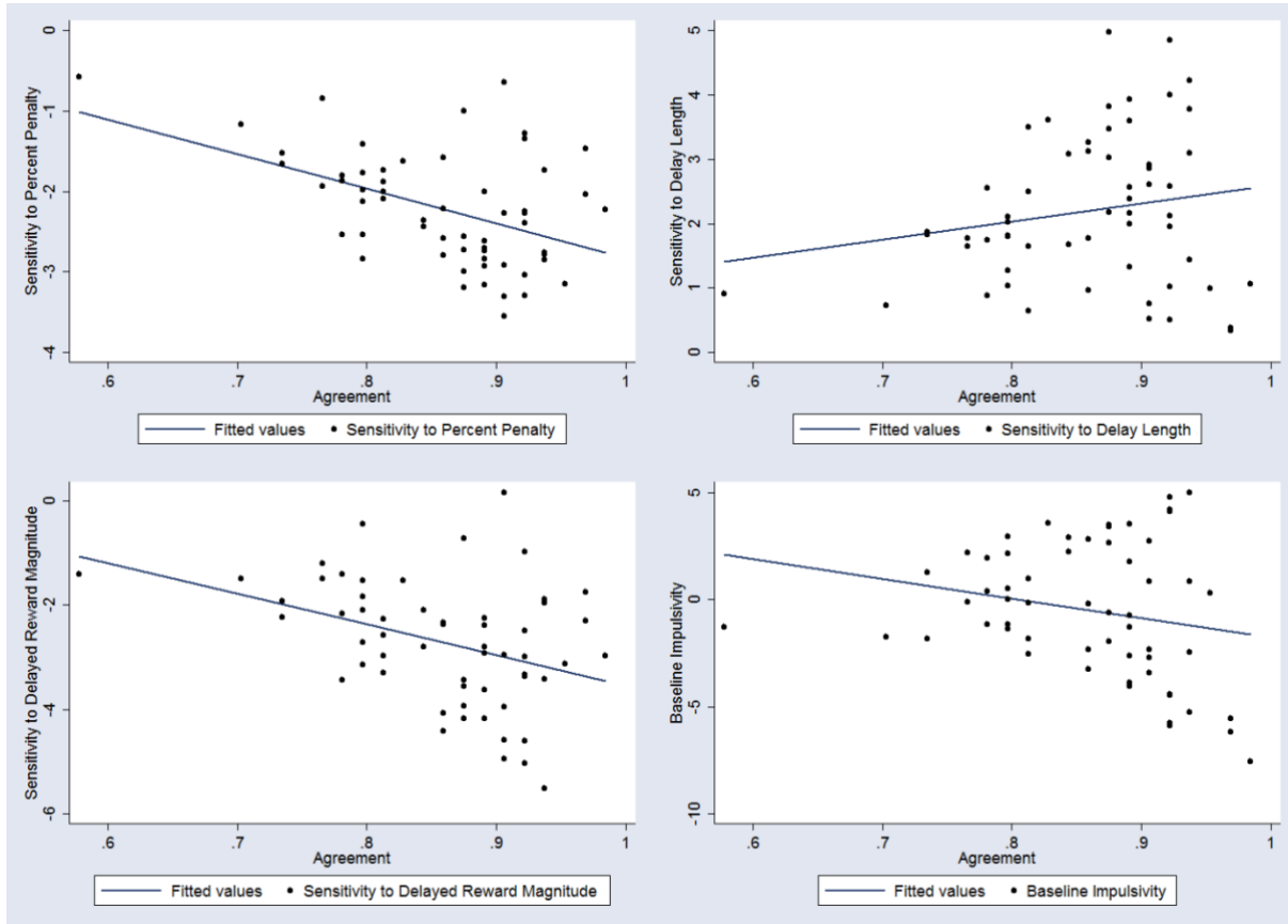
2 Supplementary Figure 4. Correlations between behavioral model estimates and choice consistency in 58 3 healthy controls who chose both smaller immediate and larger delayed rewards during the task.
