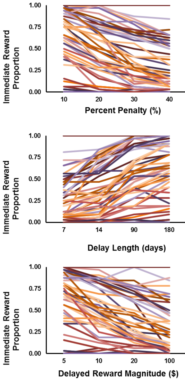
3 Supplementary Figure 1. Relationships between values of the choice attributes and the proportion of 4 smaller immediate rewards chosen by healthy controls. Each line represents an individual control's 5 decisions during the task.
